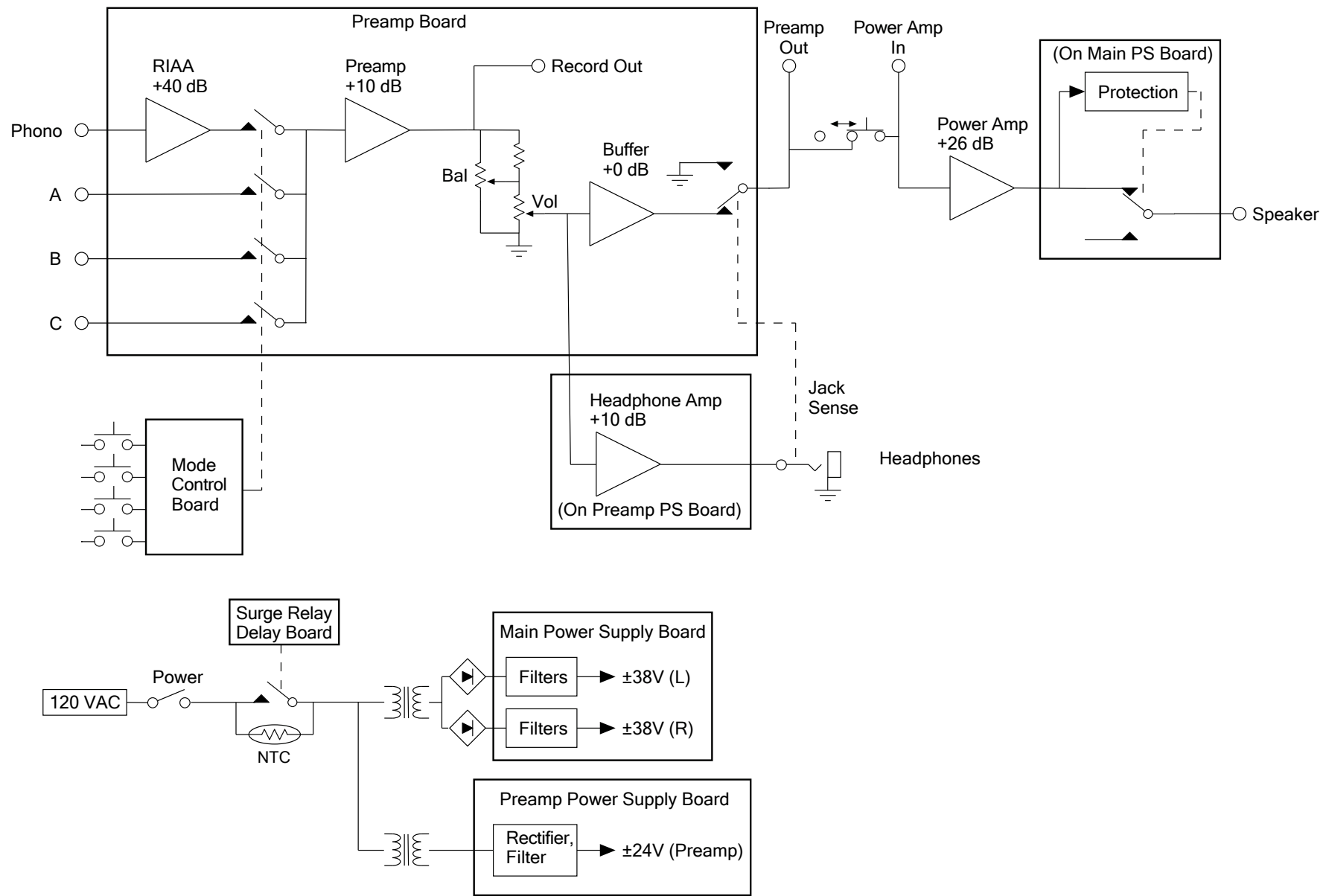
WB9JPS Integrated Amplifier Block Diagram GWJ 7-3-11 Page 1 of 1
