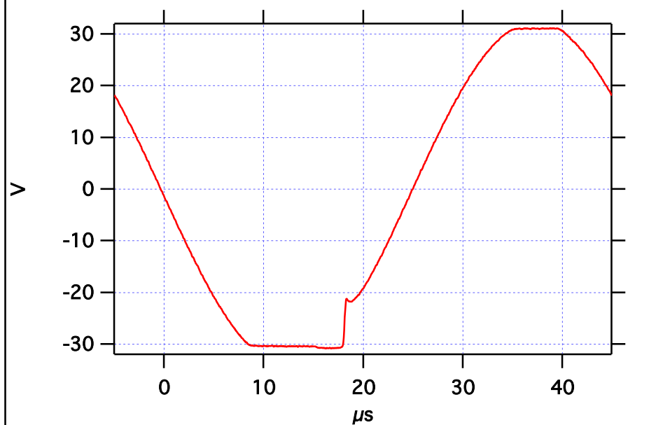
Hard Clipping, 20 kHz, 8 \Omega
