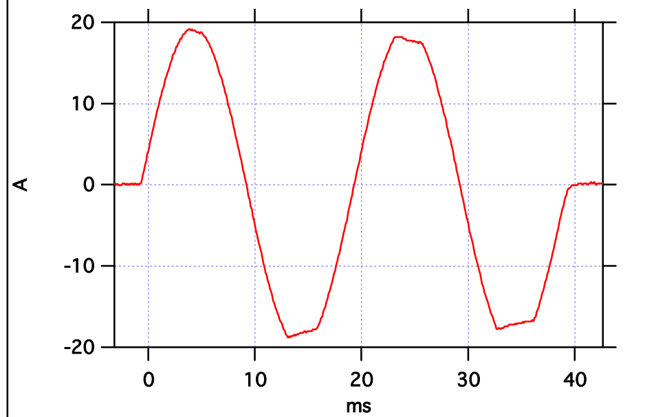
Peak Current, 50 Hz Burst, 1 \Omega Load
