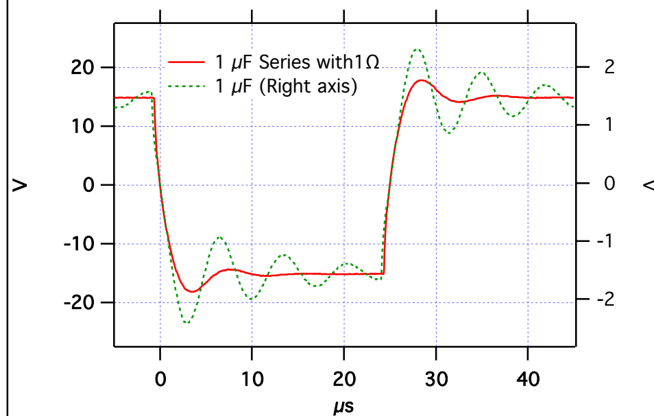
Capacitive Load Response, 20 kHz
