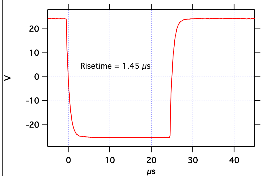
Square Wave, 8 \Omega , 20 kHz, Left (No input lowpass)
