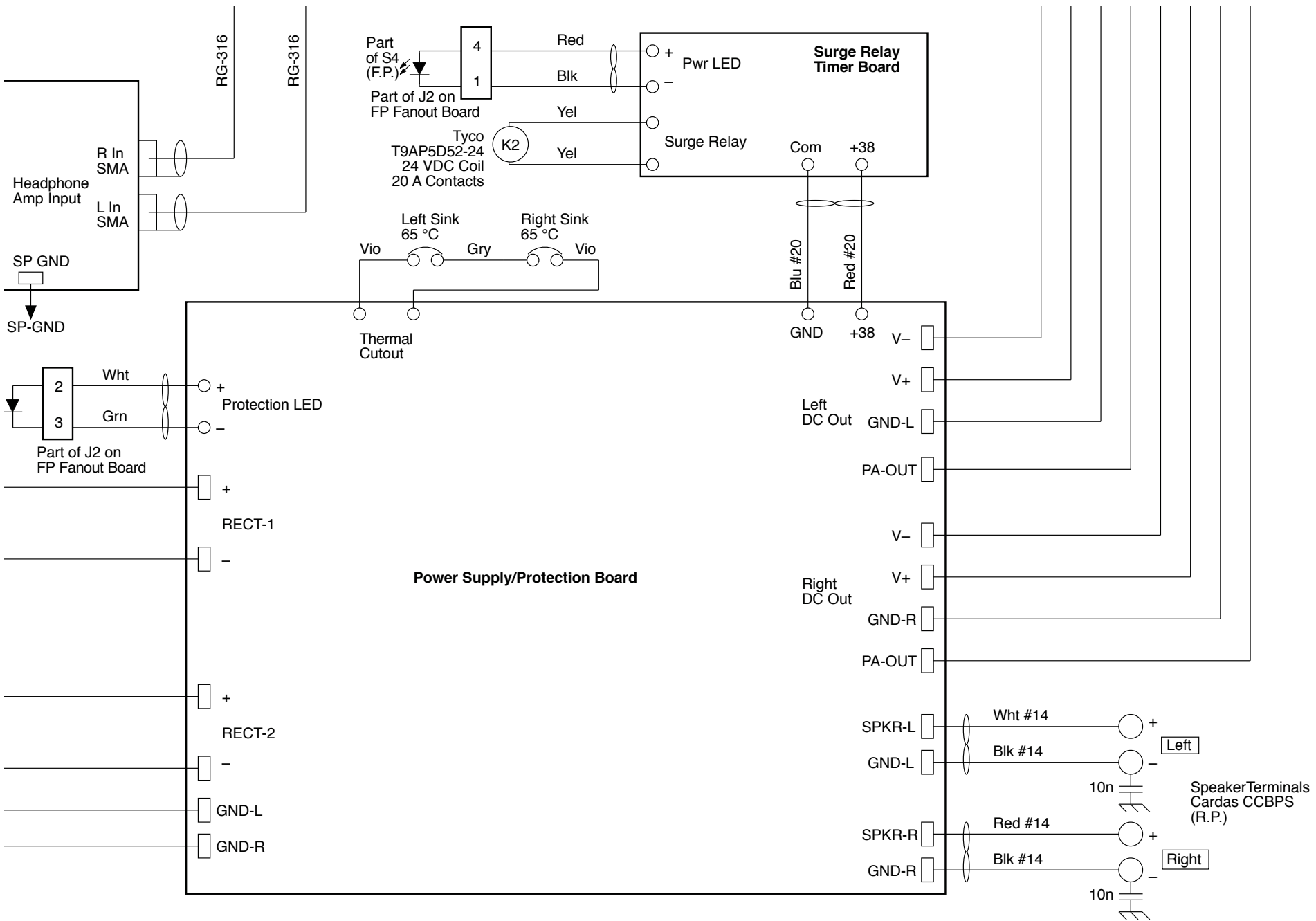
WB9JPS Integrated Amplifier System Wiring Diagram GWJ 7-3-11 Page 1 of 1
